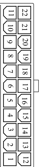
2x11P
